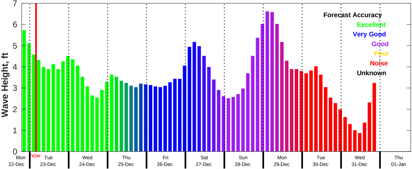
CMEMS Wave Forecast for NDBC 41013 from 22-Dec-2025 19:00:00 to 01-Jan-2026 19:00:00
