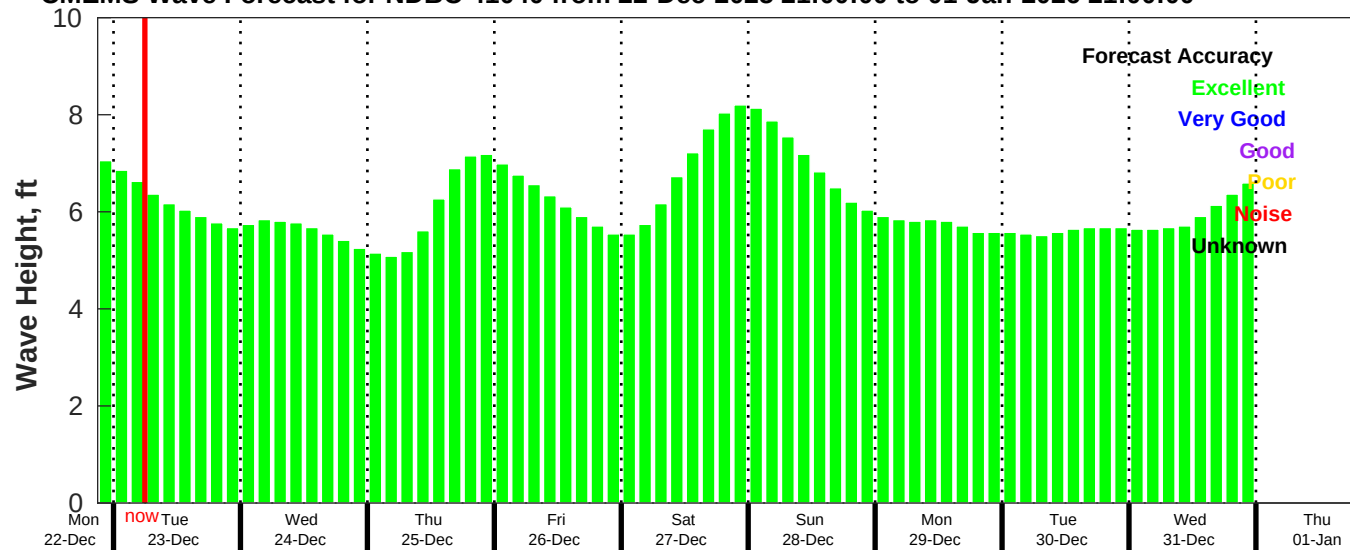
CMEMS Wave Forecast for NDBC 41040 from 22-Dec-2025 21:00:00 to 01-Jan-2026 21:00:00
