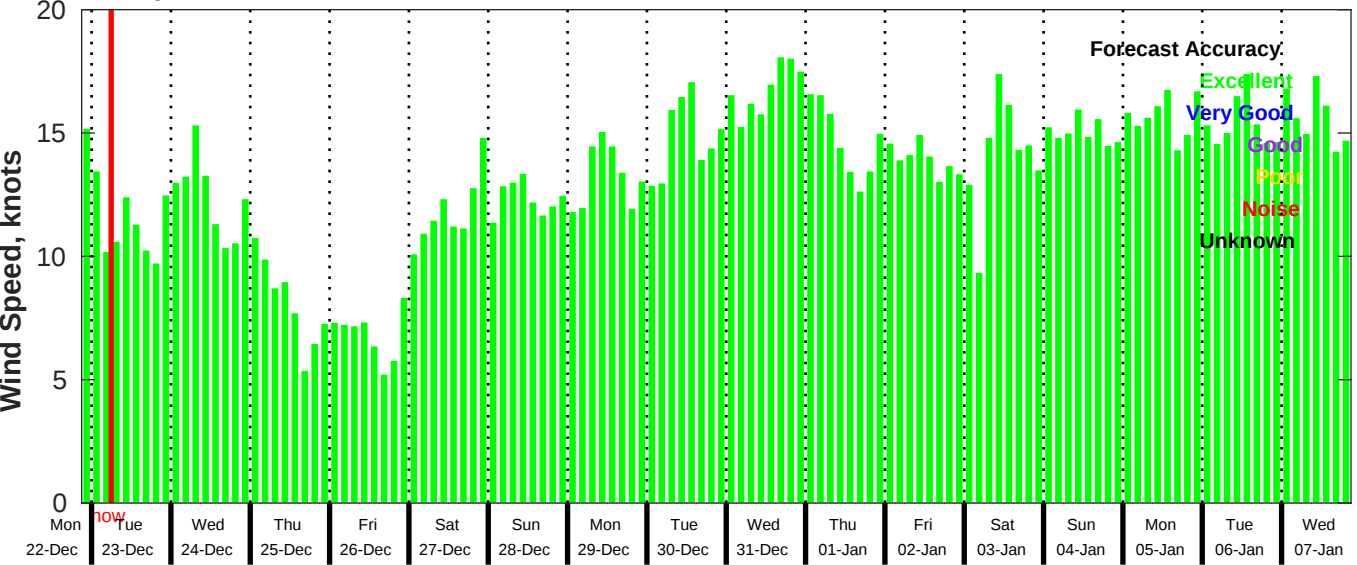
GFS Wind Speed Forecast for NDBC 41040 from 22-Dec-2025 21:00:00 to 07-Jan-2026 21:00:00
