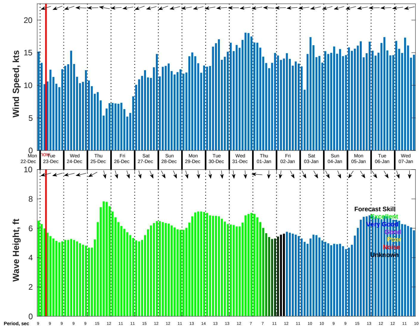
Wind & Wave Forecast for NDBC 41040 from 22-Dec-2025 21:00:00 to 07-Jan-2026 21:00:00
