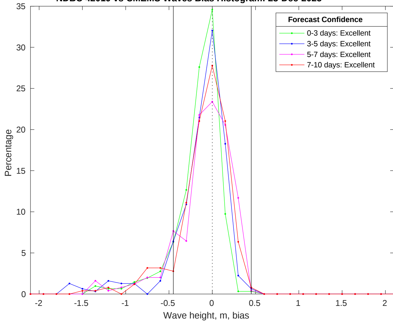
NDBC 42019 vs CMEMS Waves Bias Histogram: 23-Dec-2025
