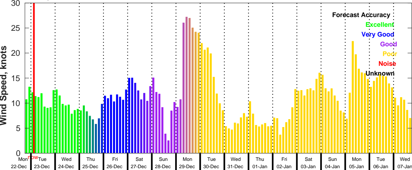
GFS Wind Speed Forecast for NDBC 42019 from 22-Dec-2025 18:00:00 to 07-Jan-2026 18:00:00
