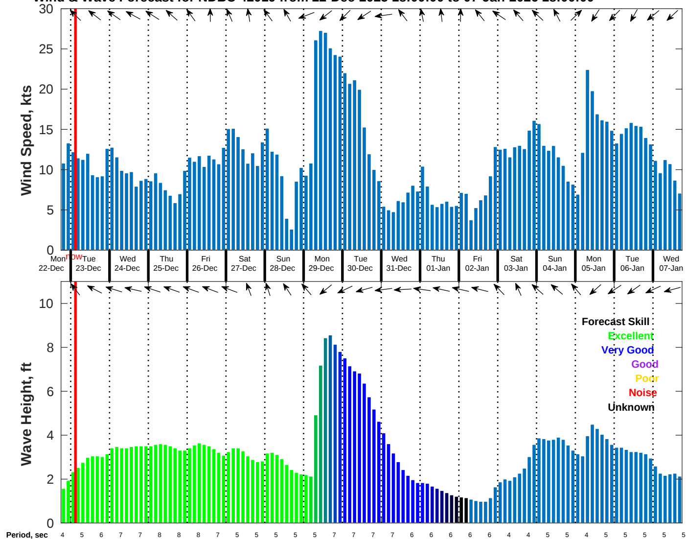
Wind & Wave Forecast for NDBC 42019 from 22-Dec-2025 18:00:00 to 07-Jan-2026 18:00:00
