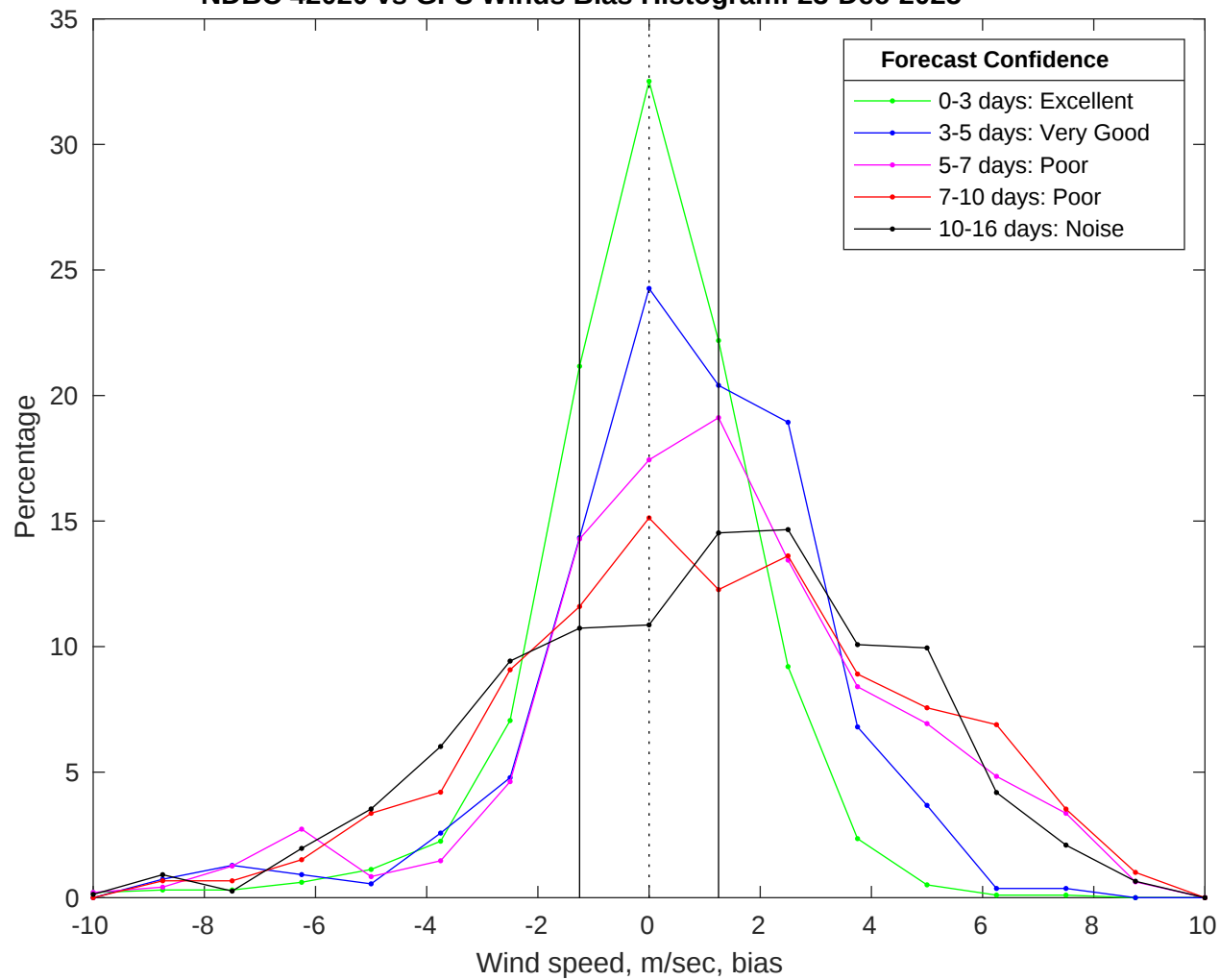
NDBC 42020 vs GFS Winds Bias Histogram: 23-Dec-2025
