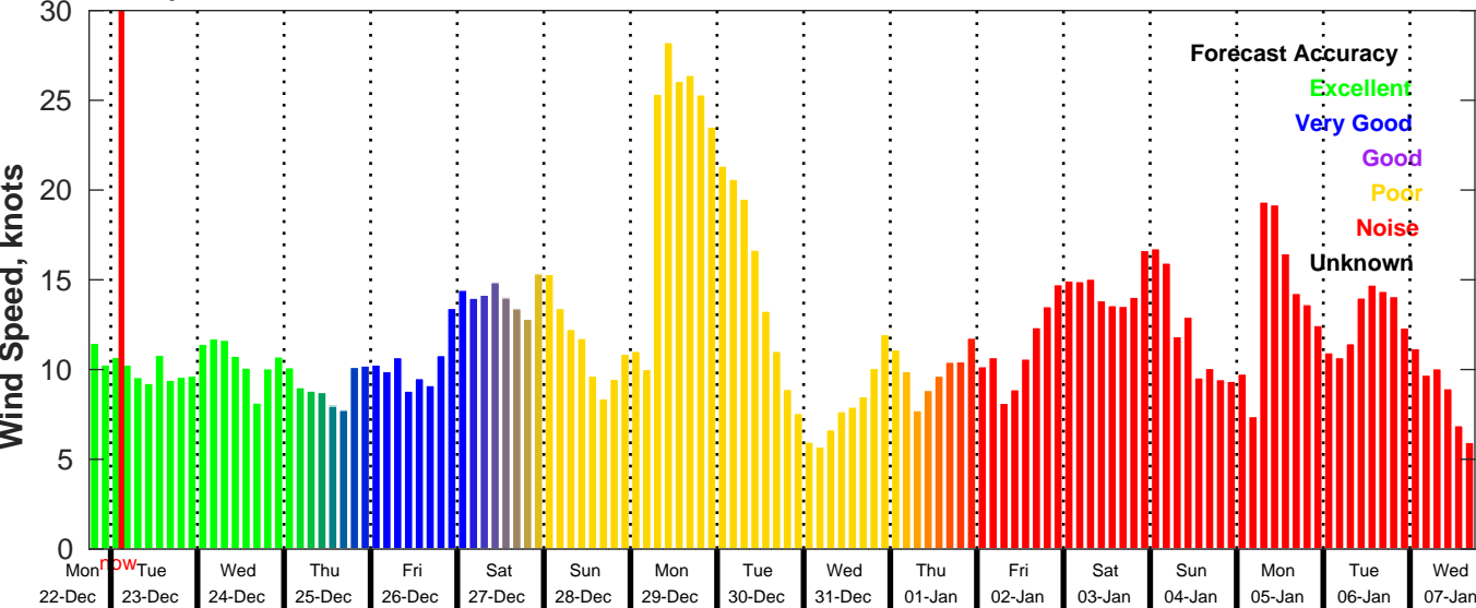
GFS Wind Speed Forecast for NDBC 42020 from 22-Dec-2025 18:00:00 to 07-Jan-2026 18:00:00
