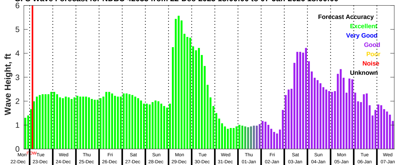
GFS Wave Forecast for NDBC 42035 from 22-Dec-2025 18:00:00 to 07-Jan-2026 18:00:00
