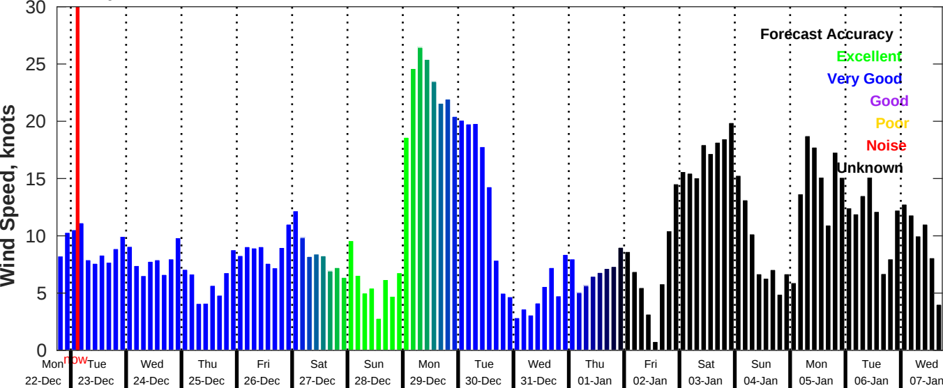
GFS Wind Speed Forecast for NDBC 42035 from 22-Dec-2025 18:00:00 to 07-Jan-2026 18:00:00
