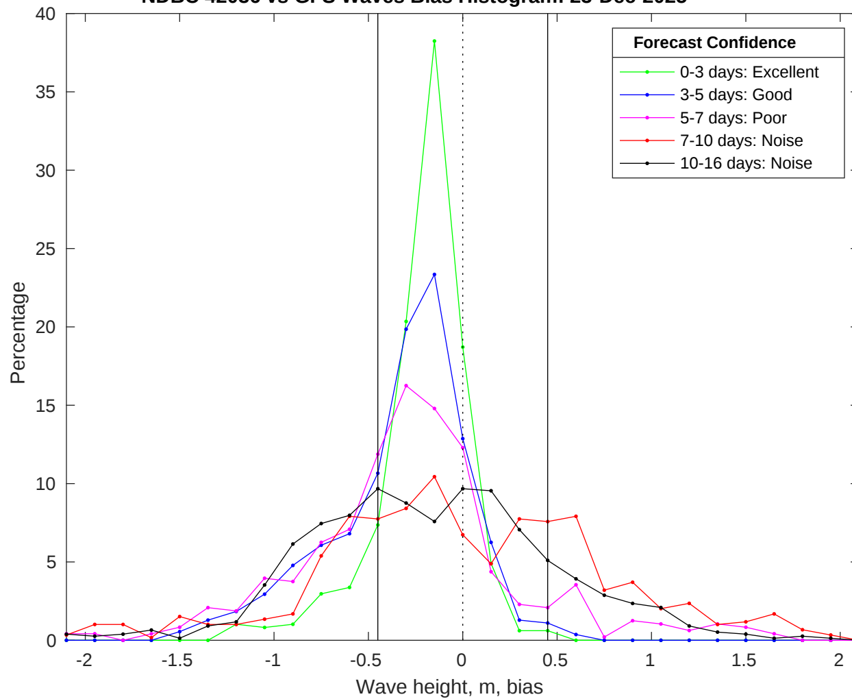
NDBC 42036 vs GFS Waves Bias Histogram: 23-Dec-2025
