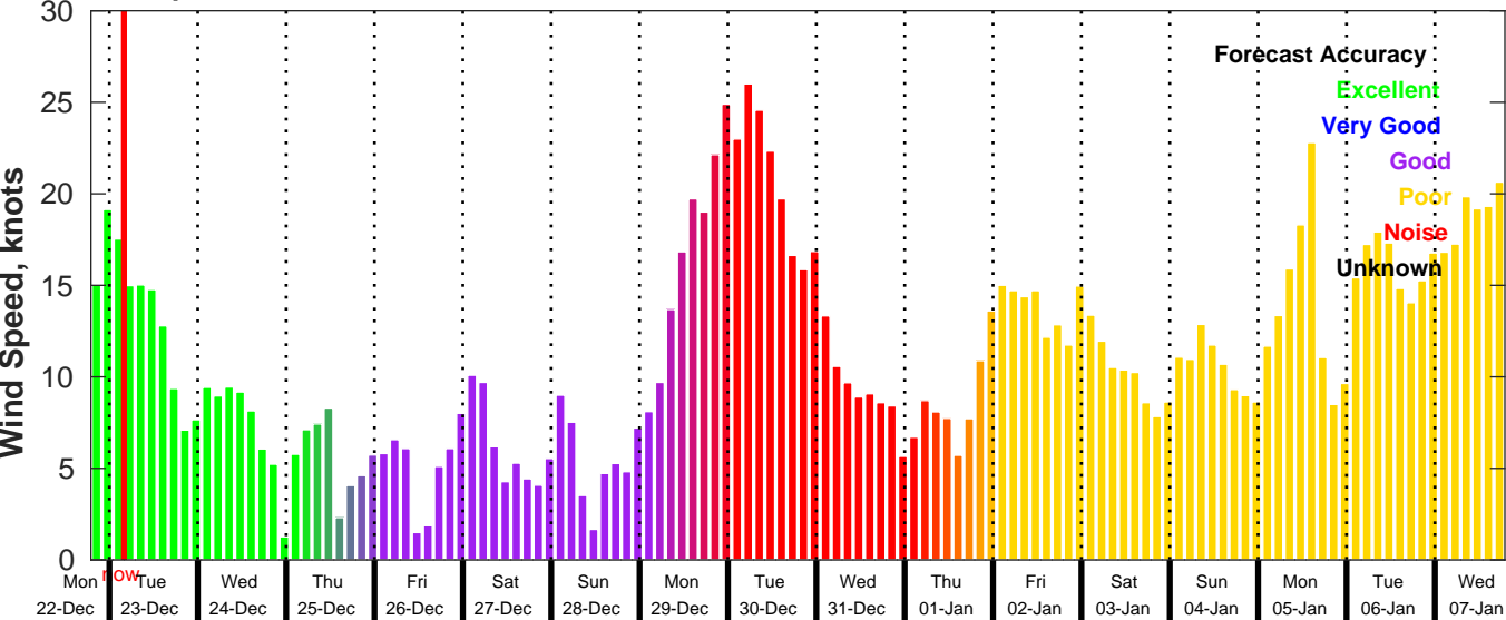
GFS Wind Speed Forecast for NDBC 42036 from 22-Dec-2025 19:00:00 to 07-Jan-2026 19:00:00
