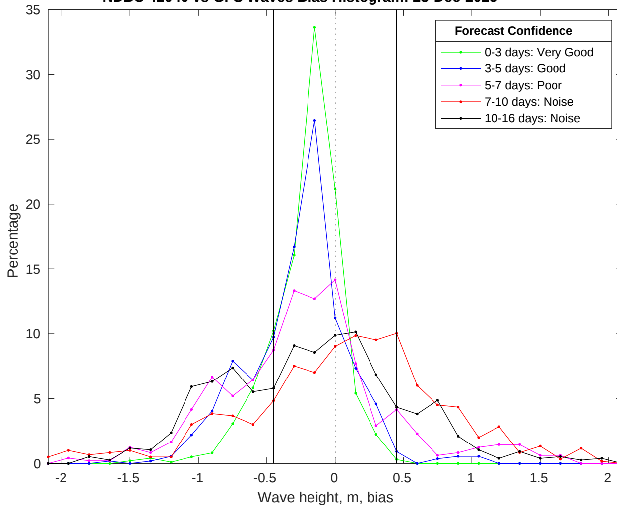
NDBC 42040 vs GFS Waves Bias Histogram: 23-Dec-2025
