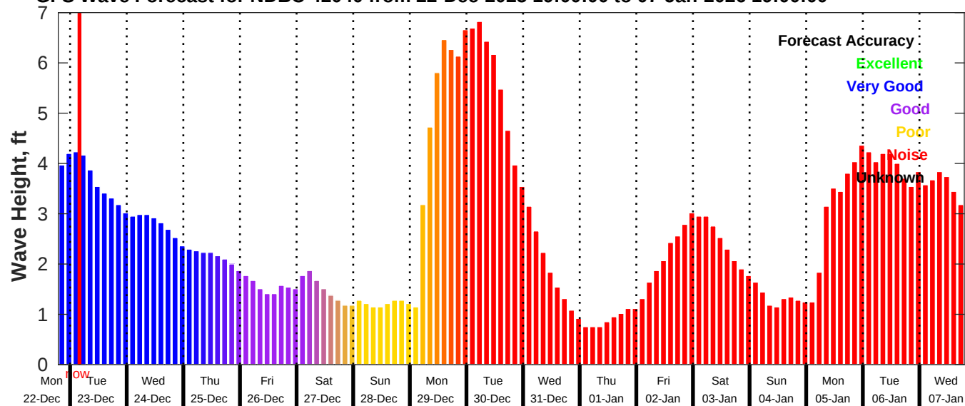
GFS Wave Forecast for NDBC 42040 from 22-Dec-2025 19:00:00 to 07-Jan-2026 19:00:00
