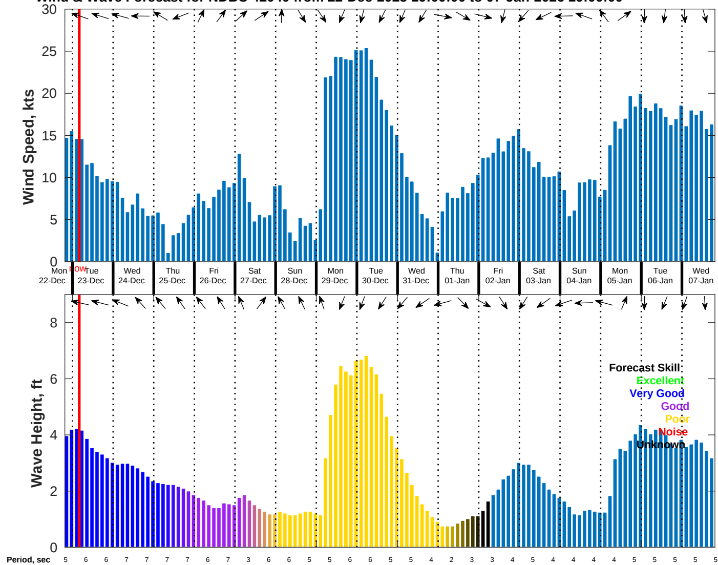
Wind & Wave Forecast for NDBC 42040 from 22-Dec-2025 19:00:00 to 07-Jan-2026 19:00:00
