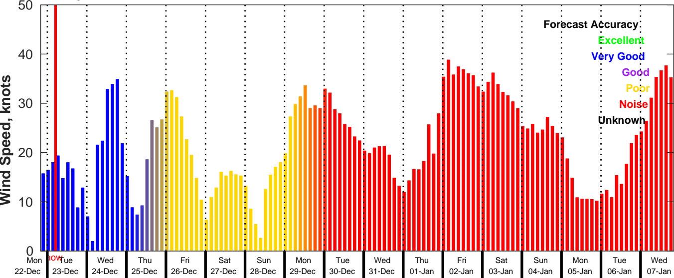
GFS Wind Speed Forecast for NDBC 44008 from 22-Dec-2025 20:00:00 to 07-Jan-2026 20:00:00
