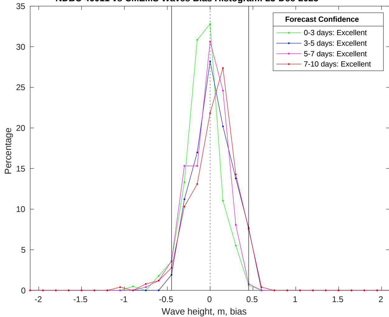
NDBC 46011 vs CMEMS Waves Bias Histogram: 23-Dec-2025
