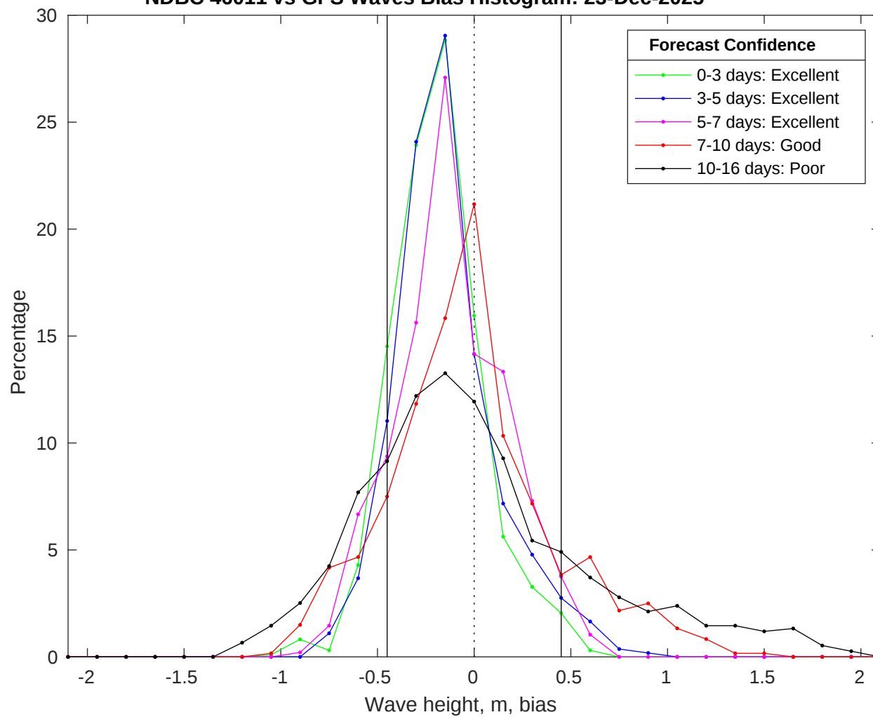
NDBC 46011 vs GFS Waves Bias Histogram: 23-Dec-2025
