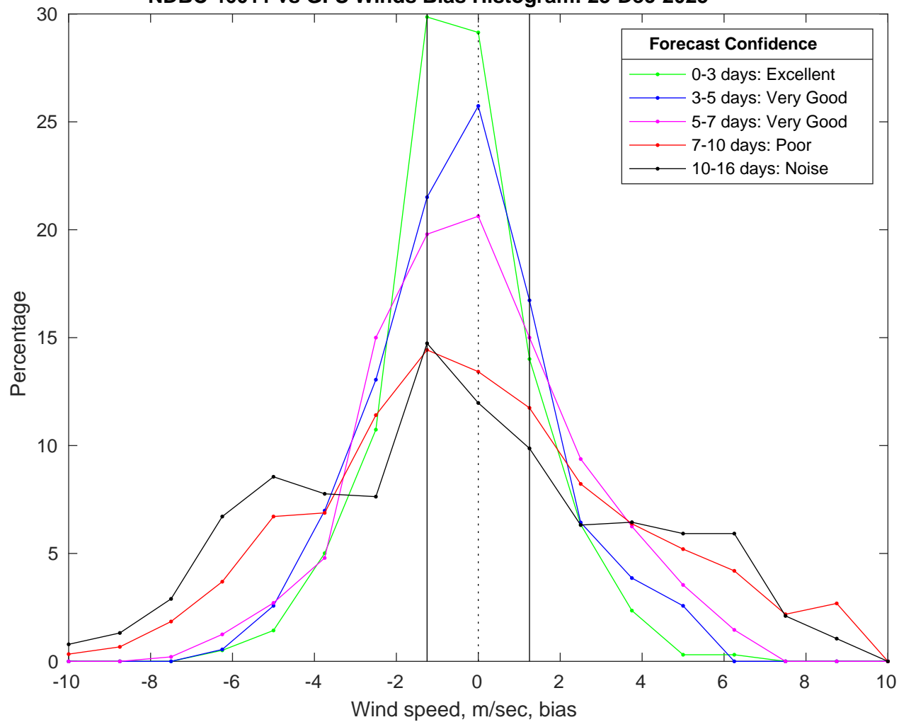
NDBC 46011 vs GFS Winds Bias Histogram: 23-Dec-2025
