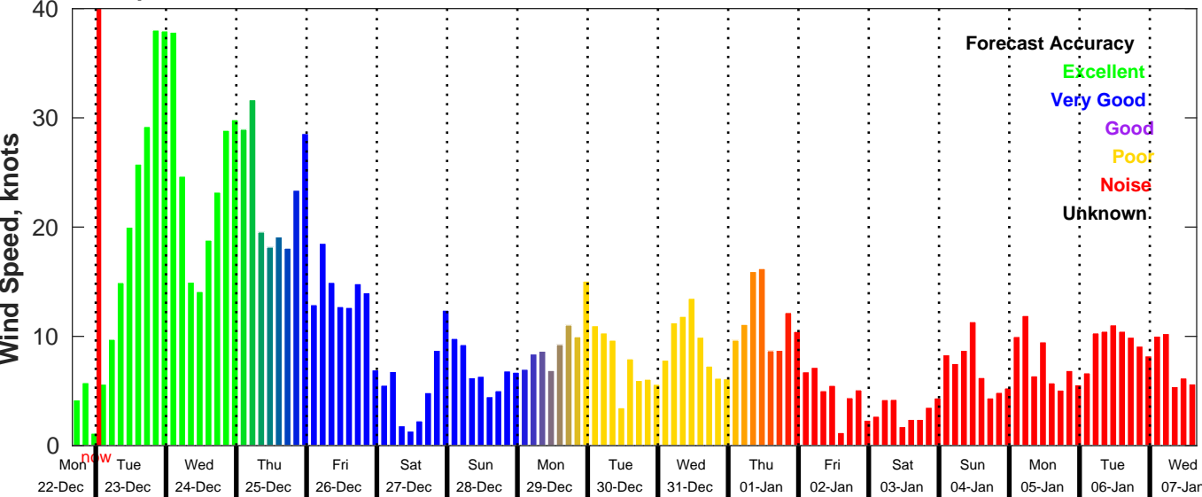
GFS Wind Speed Forecast for NDBC 46011 from 22-Dec-2025 16:00:00 to 07-Jan-2026 16:00:00
