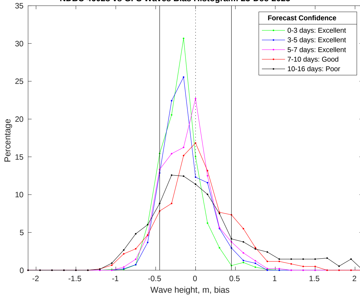
NDBC 46028 vs GFS Waves Bias Histogram: 23-Dec-2025
