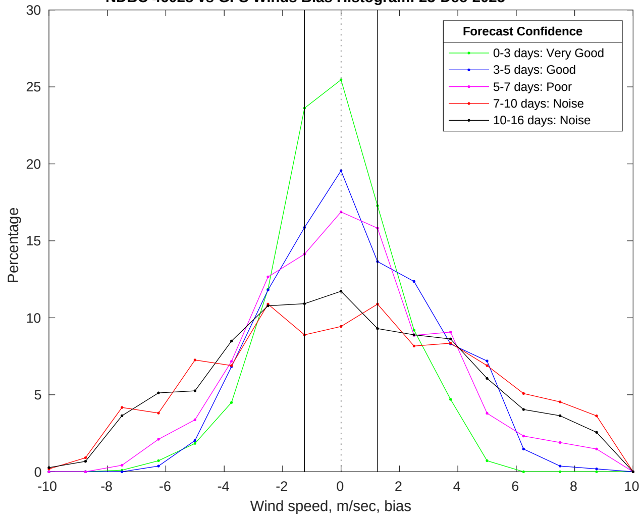
NDBC 46028 vs GFS Winds Bias Histogram: 23-Dec-2025
