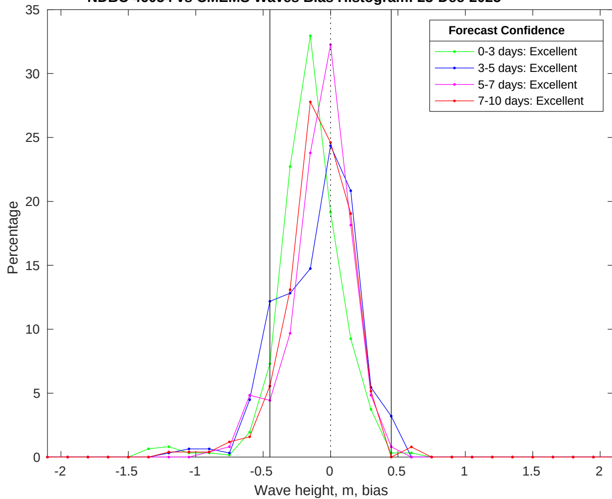
NDBC 46054 vs CMEMS Waves Bias Histogram: 23-Dec-2025
