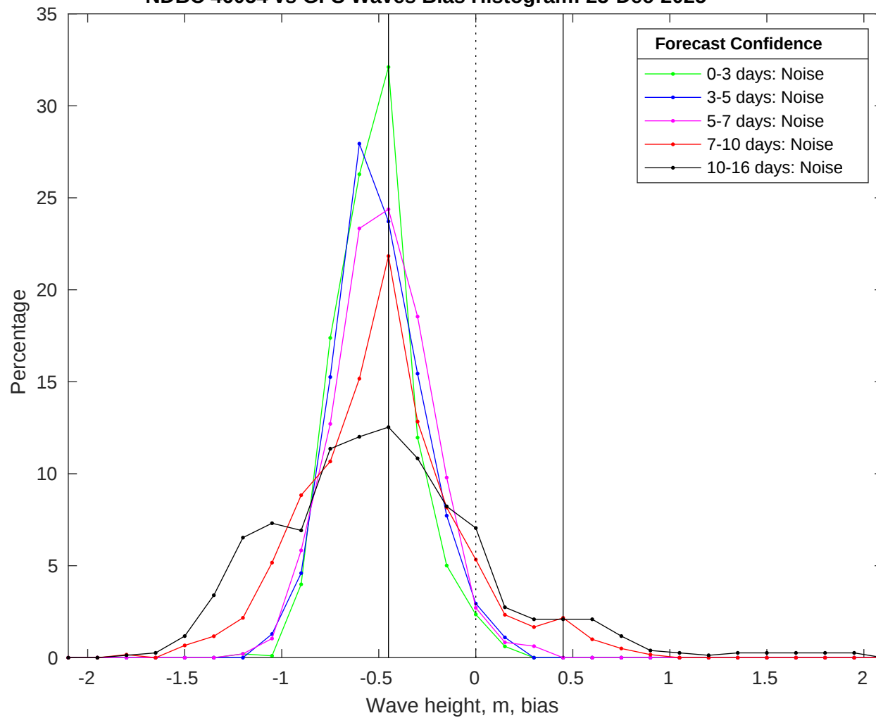
NDBC 46054 vs GFS Waves Bias Histogram: 23-Dec-2025
