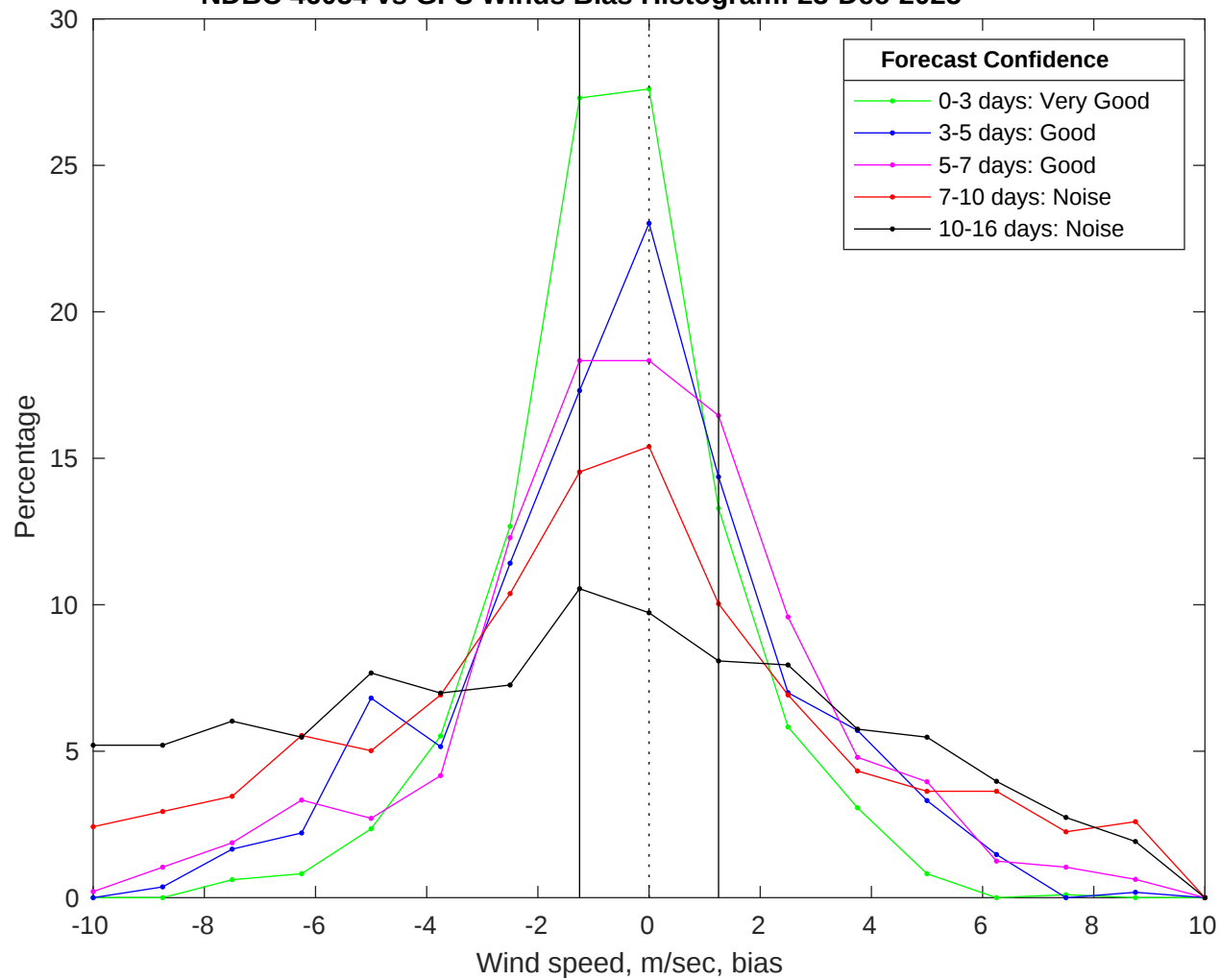
NDBC 46054 vs GFS Winds Bias Histogram: 23-Dec-2025
