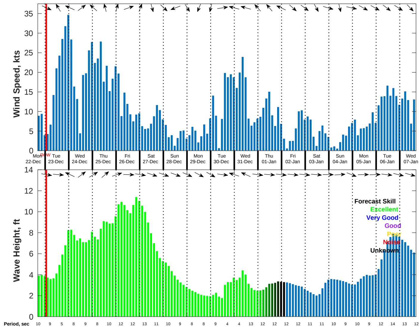
Wind & Wave Forecast for NDBC 46054 from 22-Dec-2025 16:00:00 to 07-Jan-2026 16:00:00
