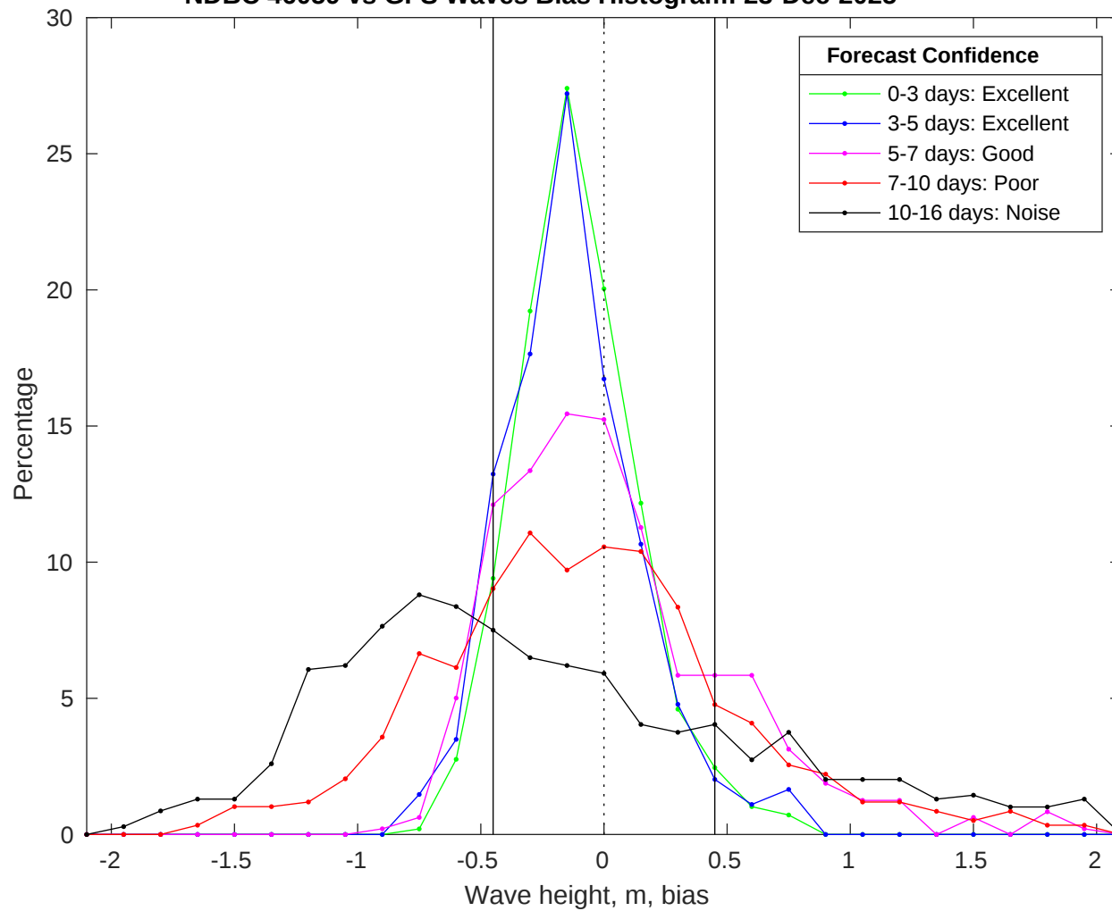
NDBC 46059 vs GFS Waves Bias Histogram: 23-Dec-2025
