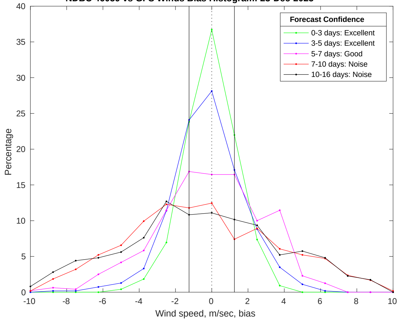
NDBC 46059 vs GFS Winds Bias Histogram: 23-Dec-2025
