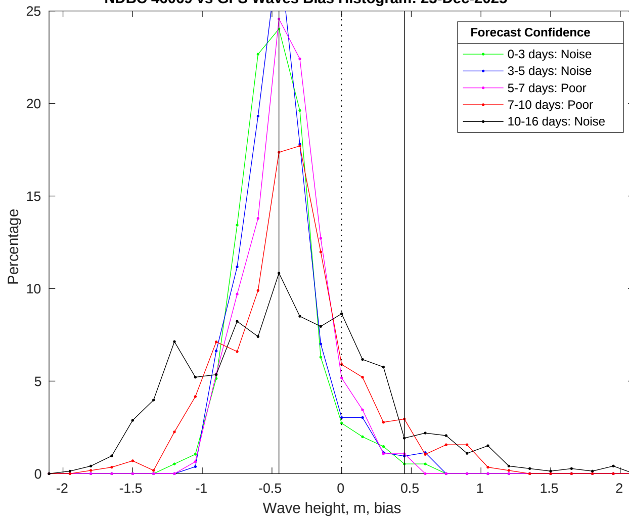
NDBC 46069 vs GFS Waves Bias Histogram: 23-Dec-2025
