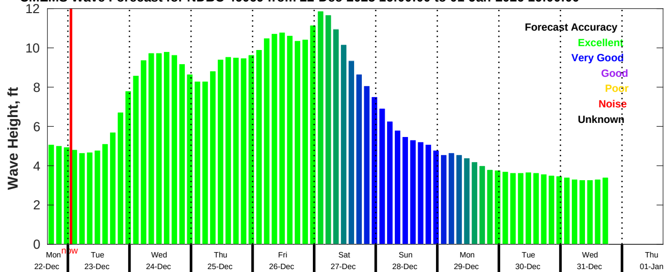
CMEMS Wave Forecast for NDBC 46069 from 22-Dec-2025 16:00:00 to 01-Jan-2026 16:00:00
