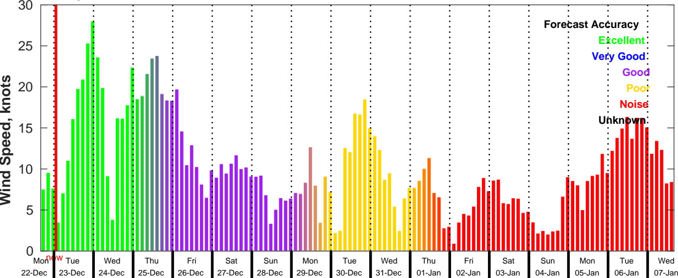
GFS Wind Speed Forecast for NDBC 46069 from 22-Dec-2025 16:00:00 to 07-Jan-2026 16:00:00
