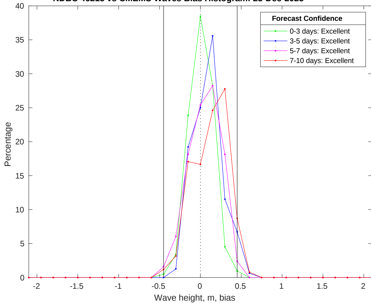
NDBC 46215 vs CMEMS Waves Bias Histogram: 23-Dec-2025
