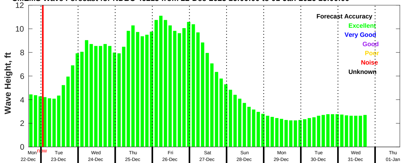
CMEMS Wave Forecast for NDBC 46215 from 22-Dec-2025 16:00:00 to 01-Jan-2026 16:00:00
