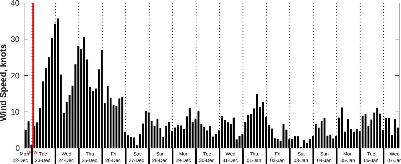
GFS Wind Speed Forecast for NDBC 46215 from 22-Dec-2025 16:00:00 to 07-Jan-2026 16:00:00
