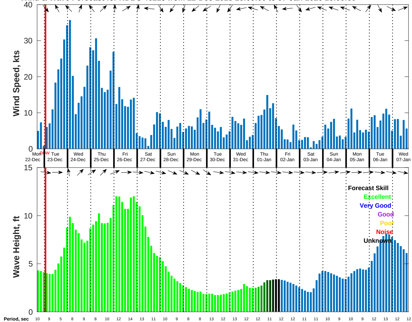
Wind & Wave Forecast for NDBC 46215 from 22-Dec-2025 16:00:00 to 07-Jan-2026 16:00:00
