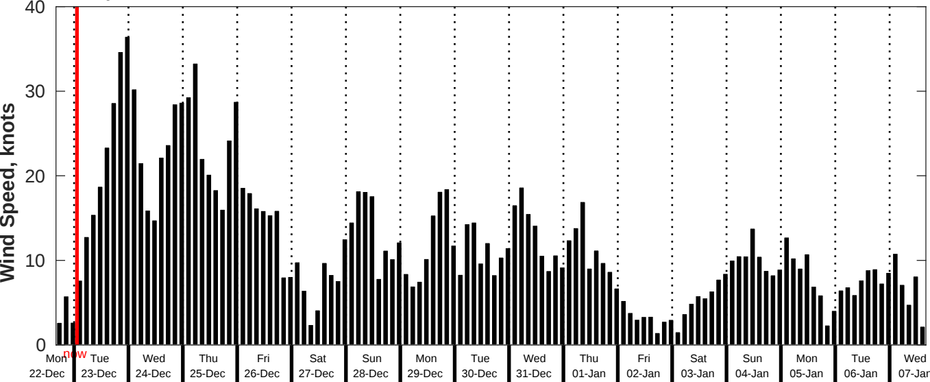
GFS Wind Speed Forecast for NDBC 46259 from 22-Dec-2025 16:00:00 to 07-Jan-2026 16:00:00
