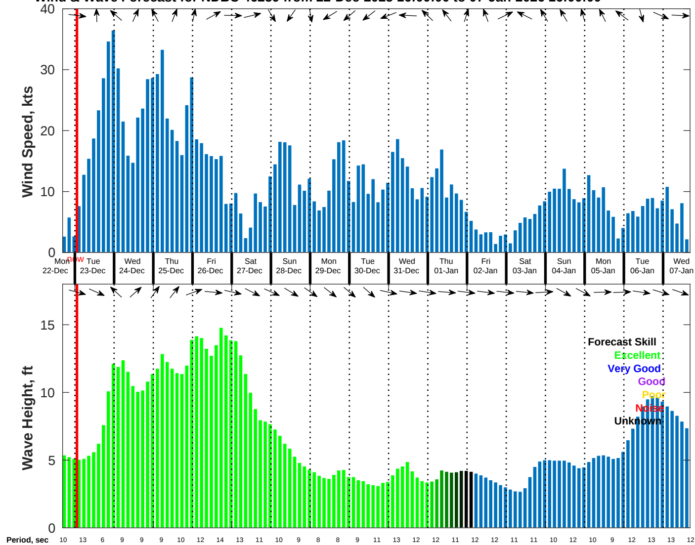
Wind & Wave Forecast for NDBC 46259 from 22-Dec-2025 16:00:00 to 07-Jan-2026 16:00:00
