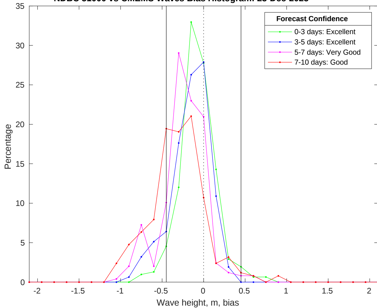
NDBC 51000 vs CMEMS Waves Bias Histogram: 23-Dec-2025
