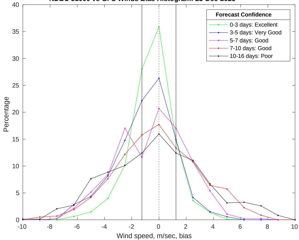
NDBC 51000 vs GFS Winds Bias Histogram: 23-Dec-2025
