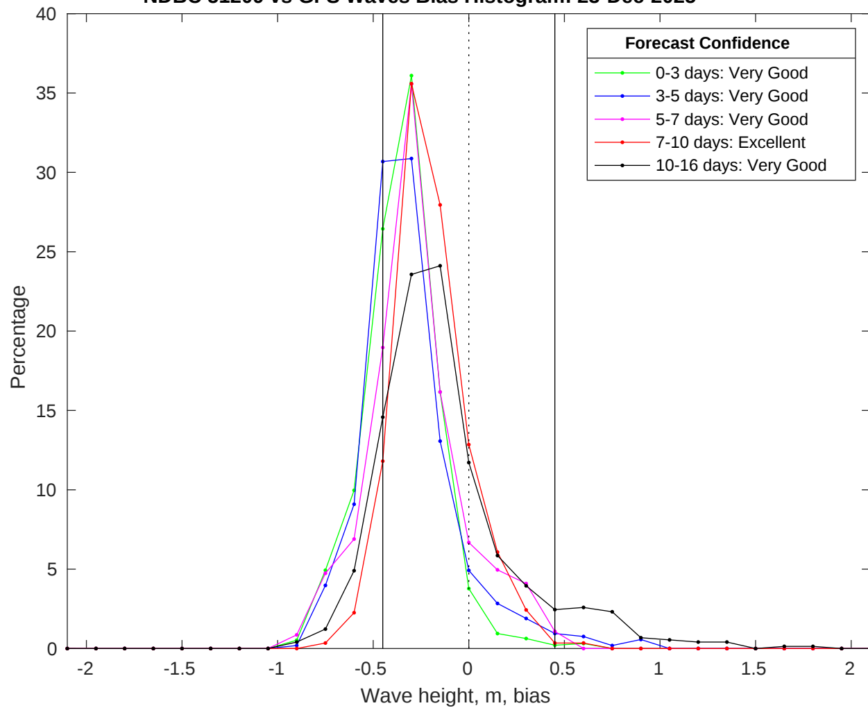
NDBC 51209 vs GFS Waves Bias Histogram: 23-Dec-2025
