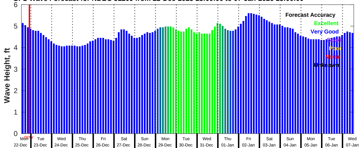
GFS Wave Forecast for NDBC 51209 from 22-Dec-2025 13:00:00 to 07-Jan-2026 13:00:00
