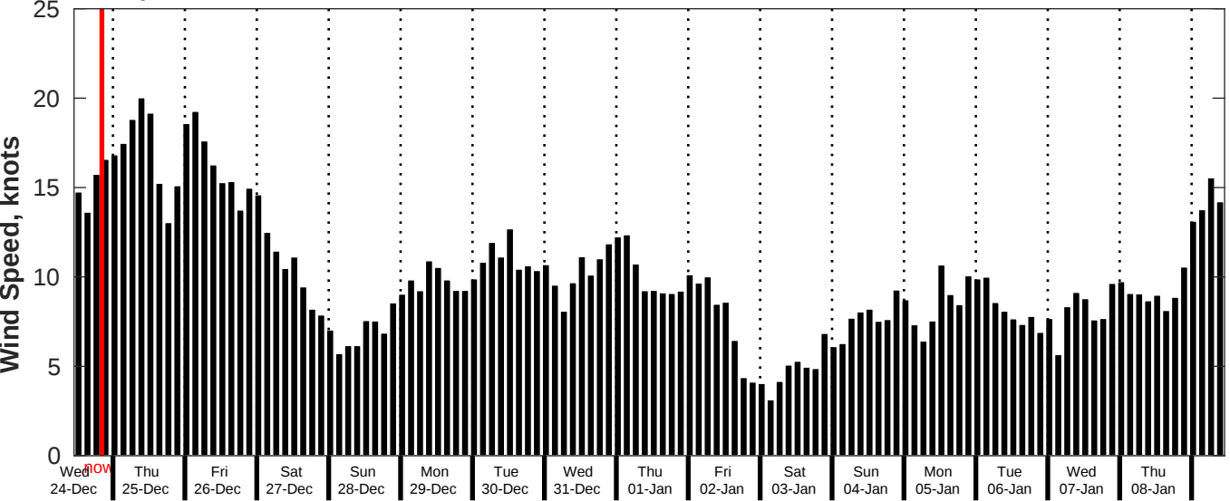
GFS Wind Speed Forecast for NDBC 52211 from 23-Dec-2025 11:00:00 to 08-Jan-2026 11:00:00
