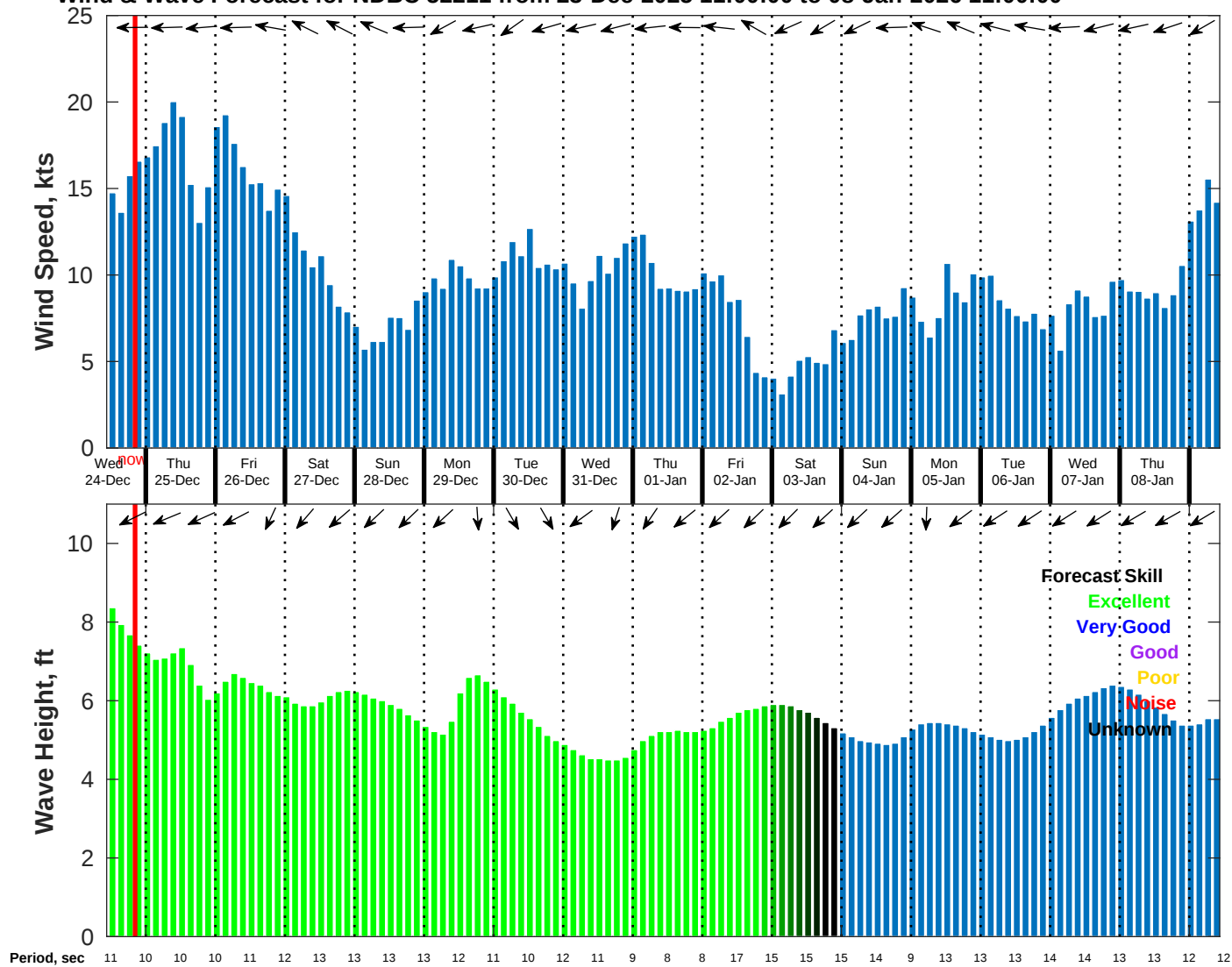
Wind & Wave Forecast for NDBC 52211 from 23-Dec-2025 11:00:00 to 08-Jan-2026 11:00:00
