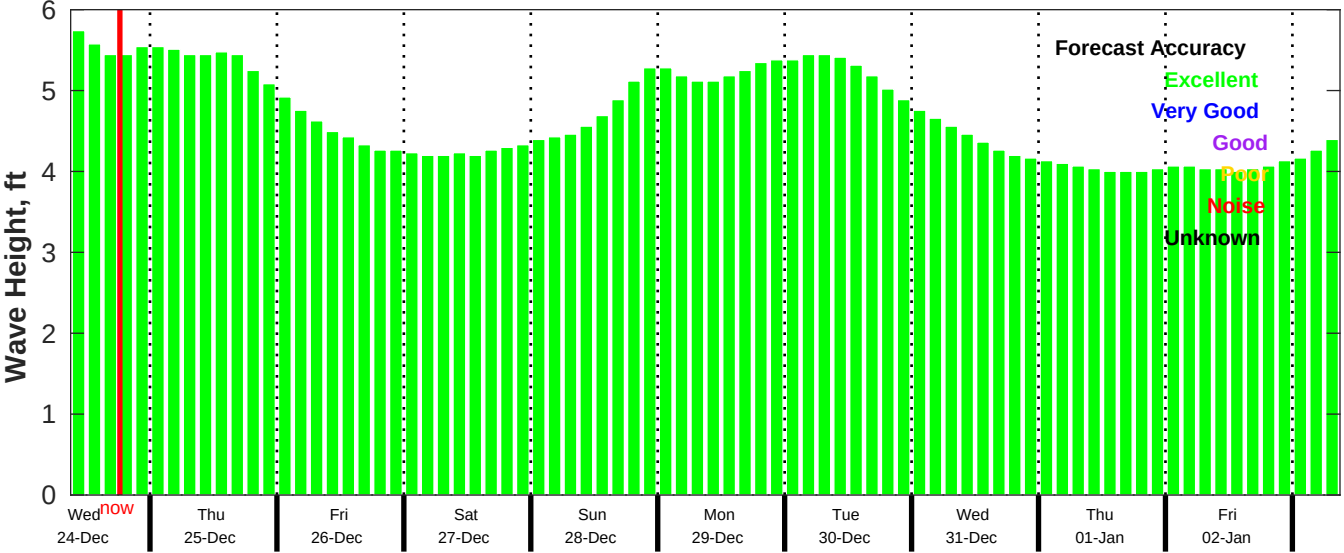
CMEMS Wave Forecast for NDBC 52212 from 23-Dec-2025 09:00:00 to 02-Jan-2026 09:00:00
