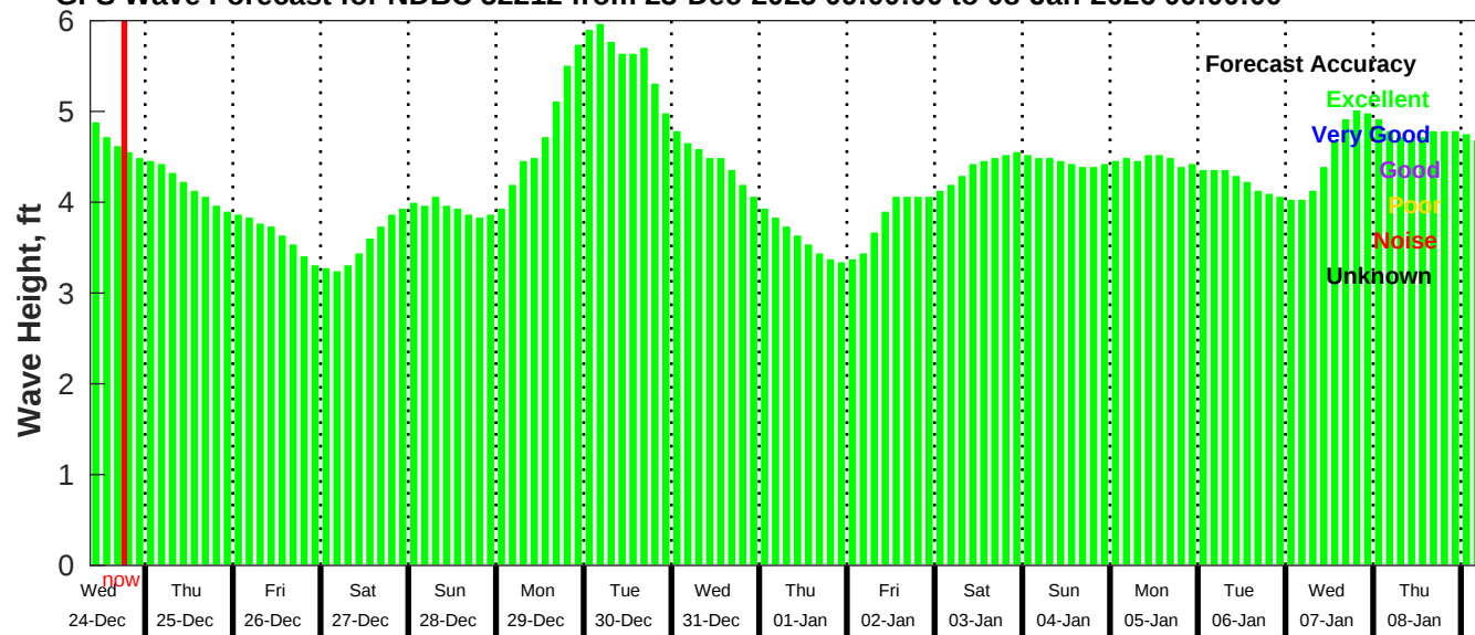
GFS Wave Forecast for NDBC 52212 from 23-Dec-2025 09:00:00 to 08-Jan-2026 09:00:00
