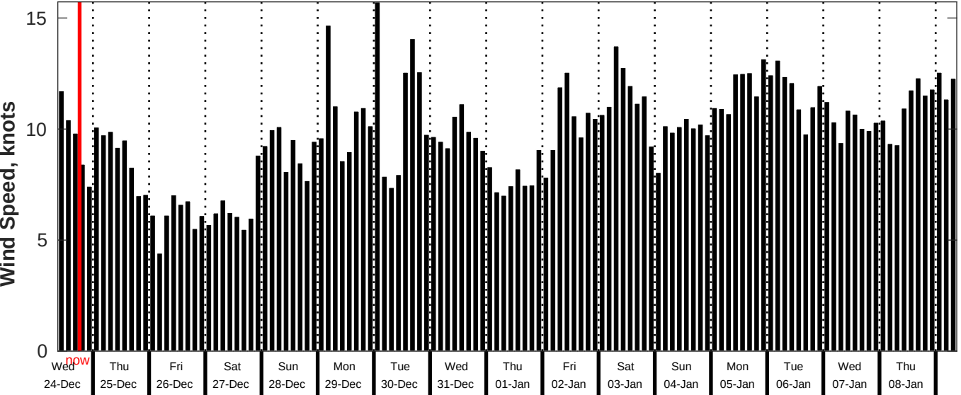
GFS Wind Speed Forecast for NDBC 52212 from 23-Dec-2025 09:00:00 to 08-Jan-2026 09:00:00
