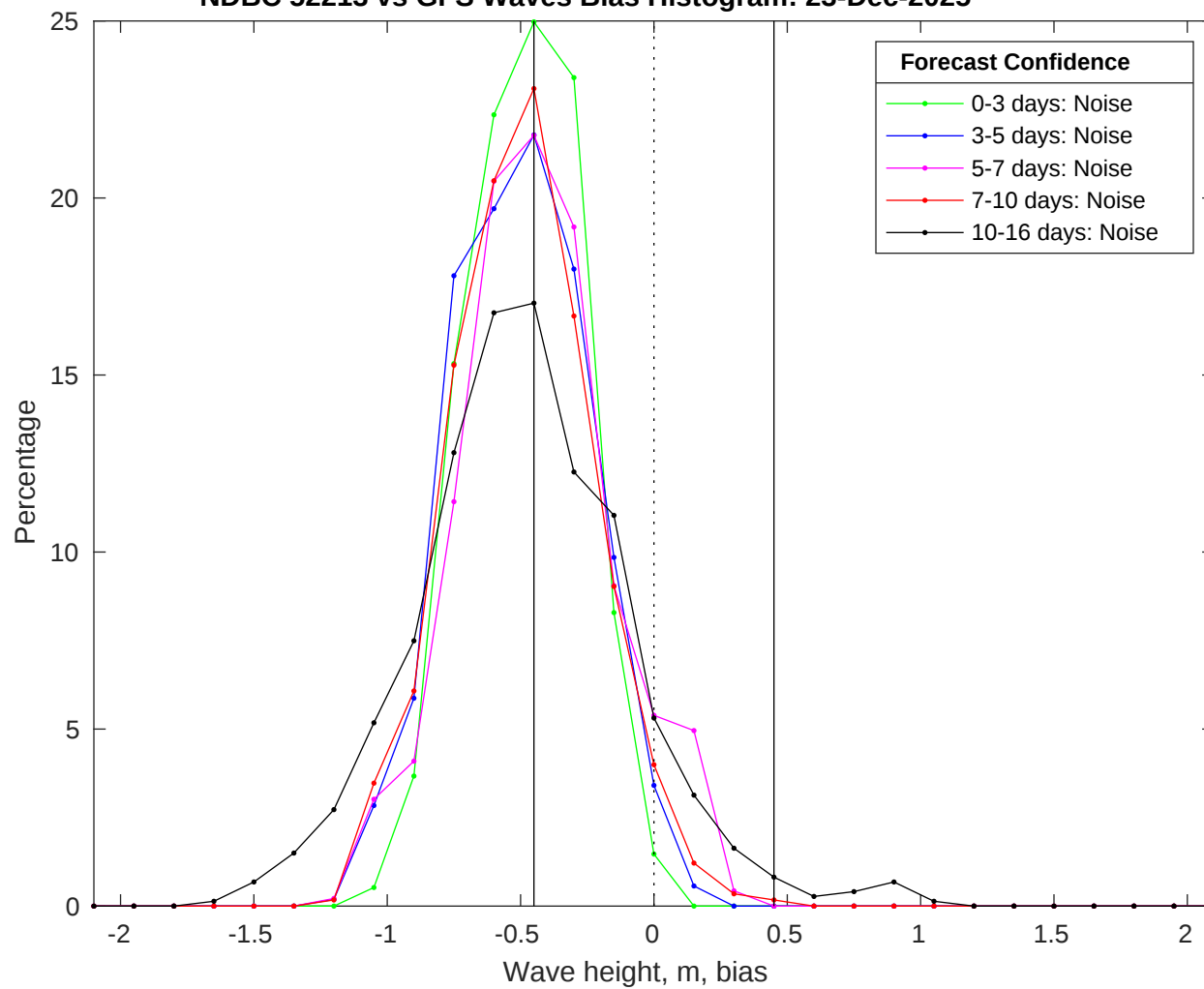
NDBC 52213 vs GFS Waves Bias Histogram: 23-Dec-2025
