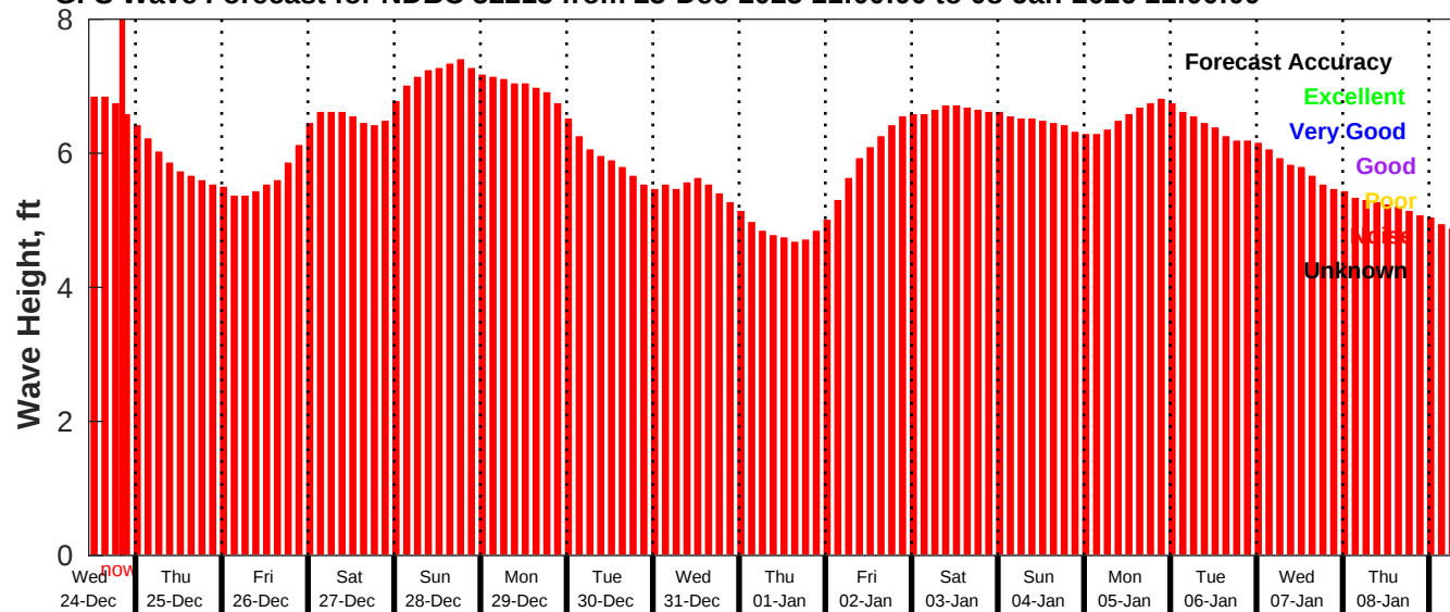
GFS Wave Forecast for NDBC 52213 from 23-Dec-2025 11:00:00 to 08-Jan-2026 11:00:00
