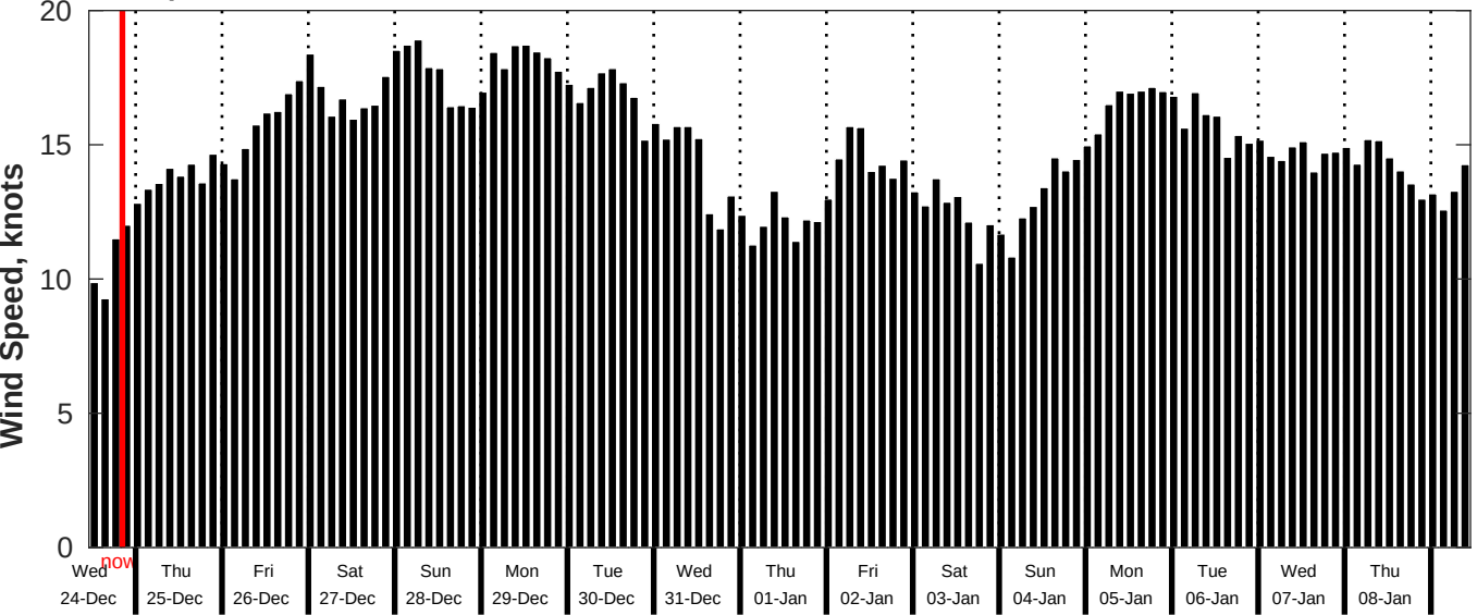
GFS Wind Speed Forecast for NDBC 52213 from 23-Dec-2025 11:00:00 to 08-Jan-2026 11:00:00
